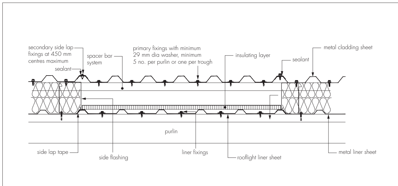
Figure 3 Fixing detail for site-assembled rooflights (cross section)
