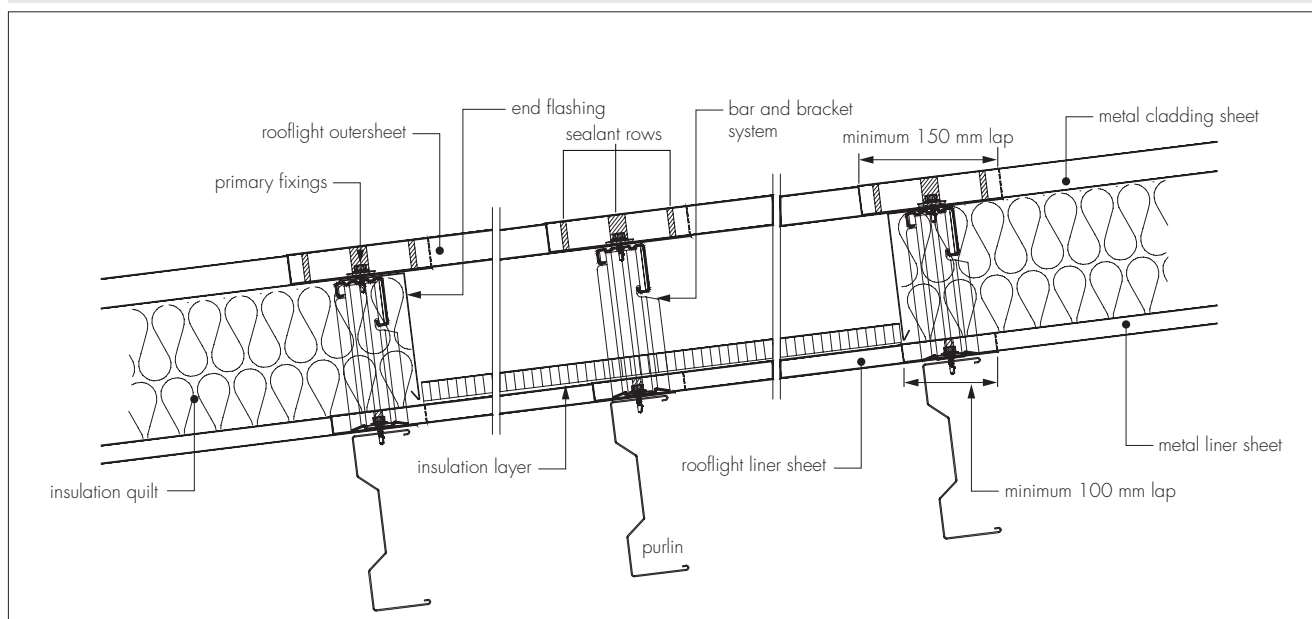
Figure 2 Fixing detail for site-assembled rooflights (along section)
