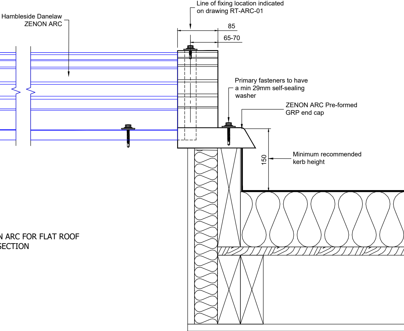
ROOFLIGHT UNDERLAP DETAIL
