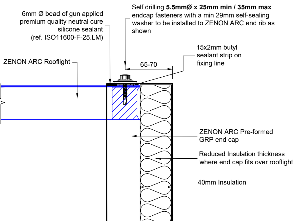
ROOFLIGHT ENDCAP OVERLAP - SECTION
