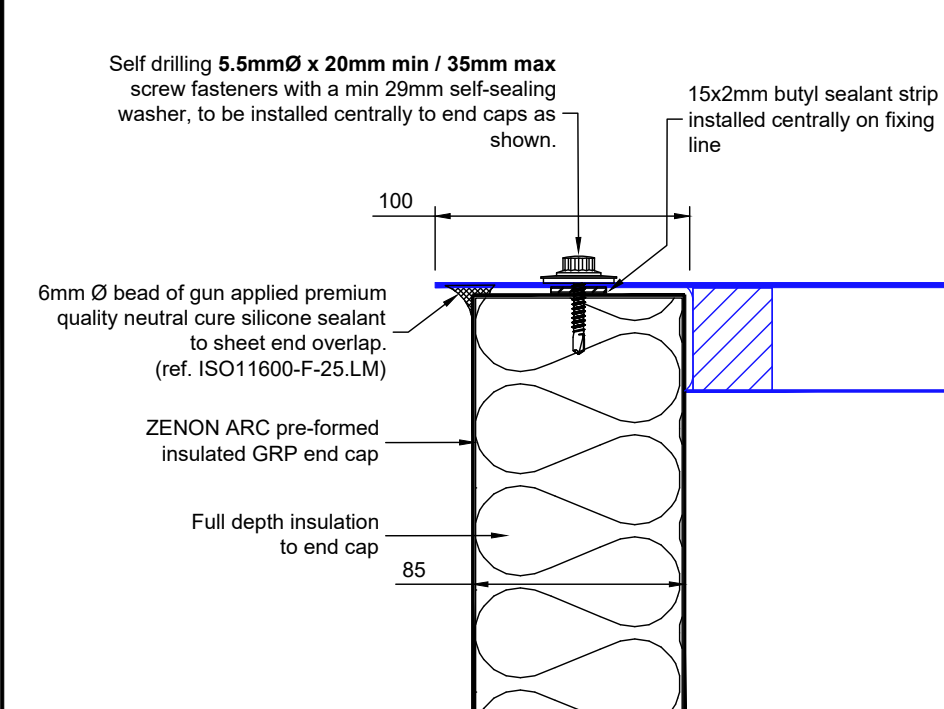
ROOFLIGHT OVERLAP ONTO ENDCAP-SECTION
