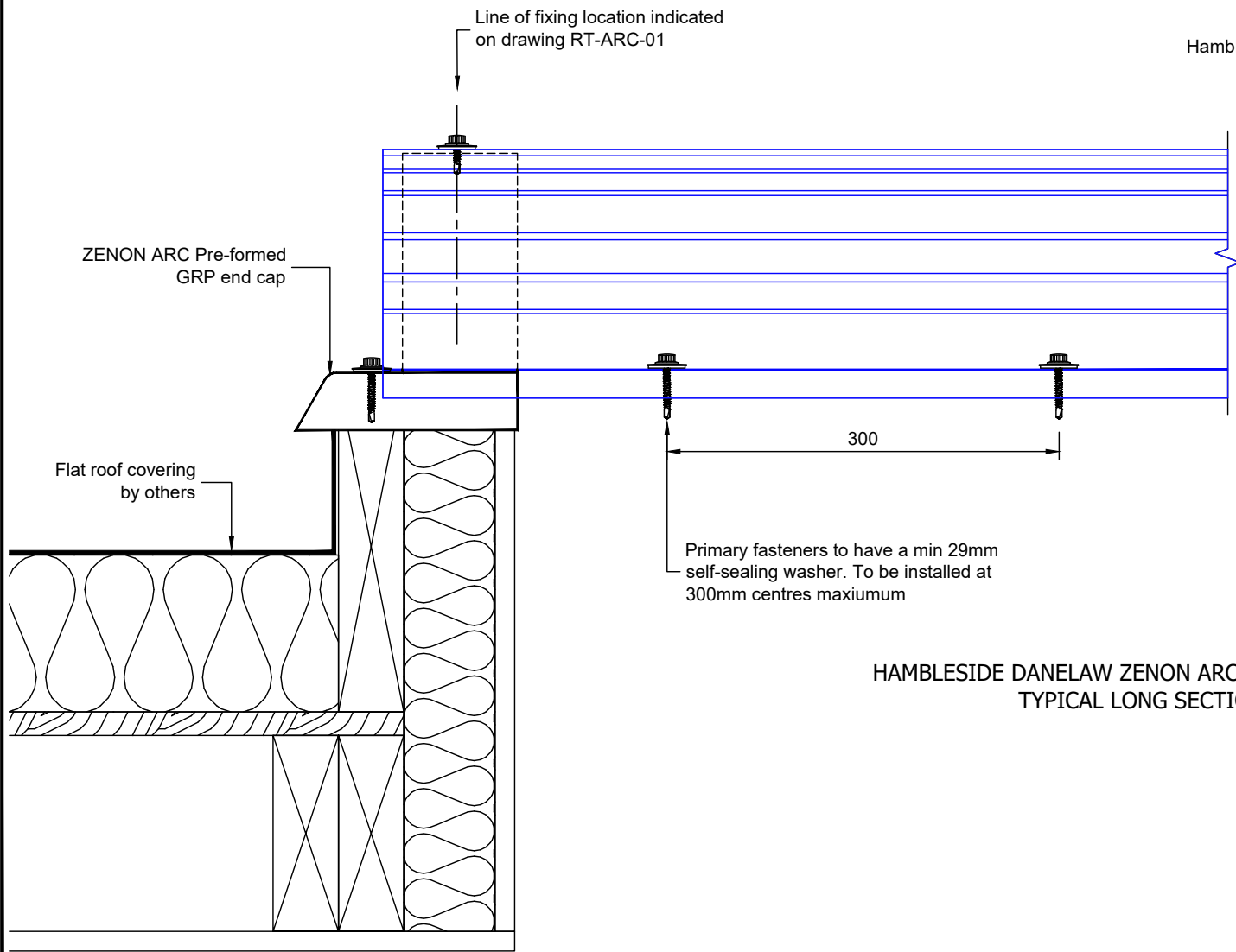
ROOFLIGHT OVERLAP DETAIL
