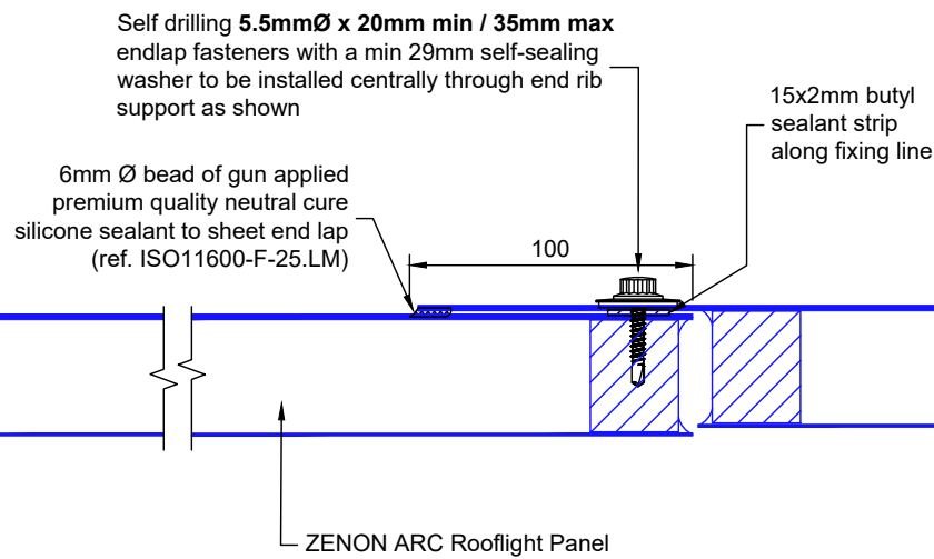
ROOFLIGHT TO ROOFLIGHT JOINT DETAIL - SECTION
